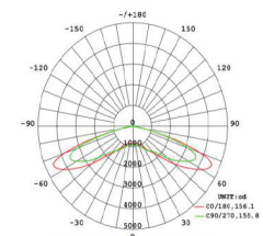
Type V (R01201) Average Beam Angle: 155.9°
