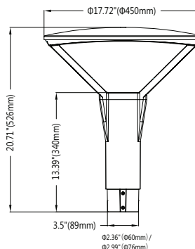
Type V (R01201) Average Beam Angle: 155.9°
